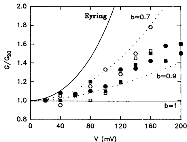
FIGURE 7 The normalized conductance-voltage relationship of solvent-free ( \circ , \square ) and decane-bilayers ( \bullet , \blacksquare ) from MGDG/DGDG/SQDG/PG mixtures. The G_{\text{H/OH}} ( \square , \blacksquare ) was measured in symmetrical pH 7.75, and the total membrane conductance G_m ( \circ , \bullet ) was measured in symmetrical 150 mM KCl, 10 mM Hepes (pH 7.2). The dotted lines were calculated from Eq. 1 with b = the fraction of the membrane spanned by the minor base of the trapezoid. Each point represents the mean of one to six experiments.
