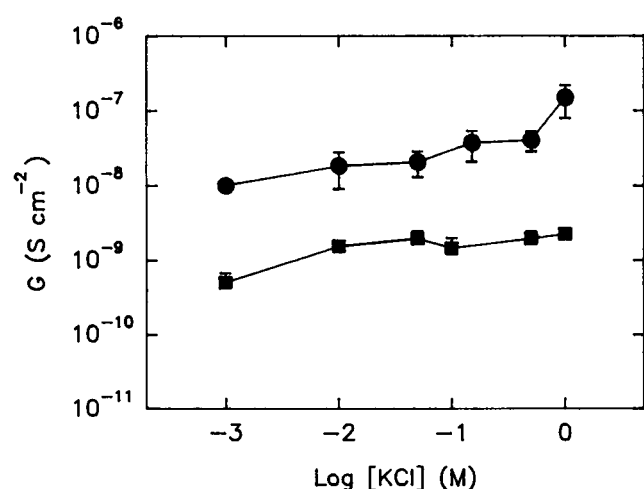
FIGURE 2 Specific conductance of decane-MGDG (●) and decane-soybean lecithin (■) as a function of the KCl concentrations of the bathing medium. The buffer used was 10 mM HEPES (pH 7.2). All conductances were determined with a potential of 60 mV.
